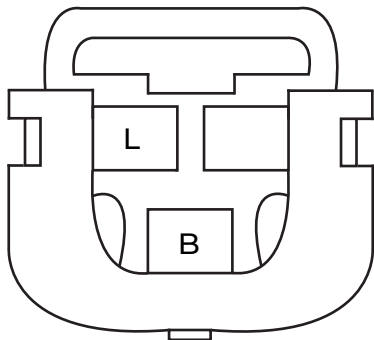
A1 Power outlet 3-pin connector (MX-30 DR : 0921 - 101)
